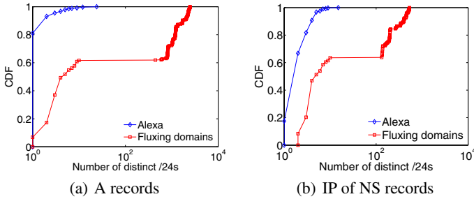
Fig. 6. Distribution of unique /24s that appeared for all records in a reply
