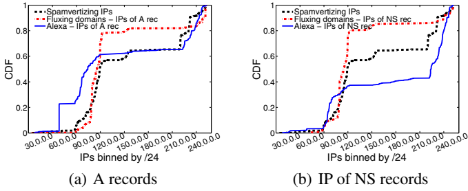
Fig. 5. Distribution of the IPs of A records of authoritative servers spam senders
