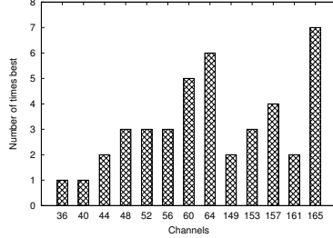
(d) Number of times each channel is best based on the RSS values on each link in the 802.11a testbed.
