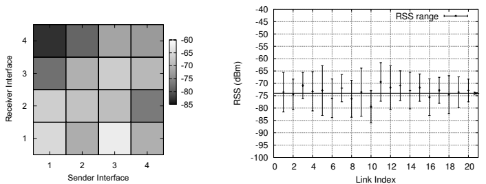
(a) RSS values (in dBm) for 16 possible interface pair combinations on a sample link.
