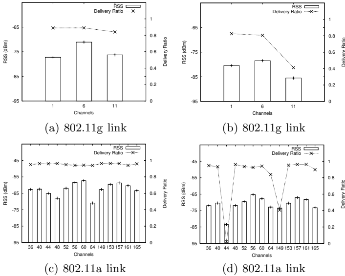
Fig. 2. Variation of RSS and delivery ratio using different channels on sample links in our two testbeds
