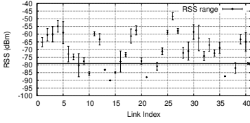
(a) Range of RSS variation in each link in 802.11g testbed across all 3 orthogonal channels.
